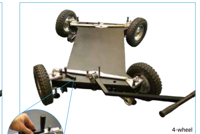
park position for crank handle
